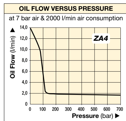
ZA4-Series Pumps with 10, 20 and 40 litres reservoir
