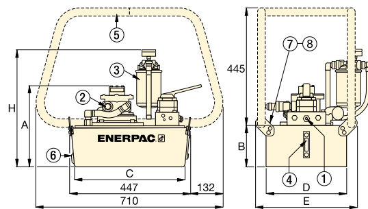
ZA4-Series Pumps with 10, 20 and 40 litres reservoir
