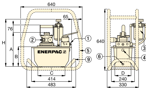
ZA4-Series Pumps with 4 - 6,6 litres reservoir
