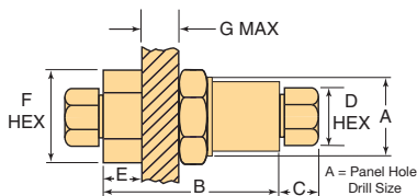
Bulkhead Coupling
