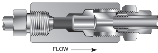
CF Series Cup Type Line Filters
