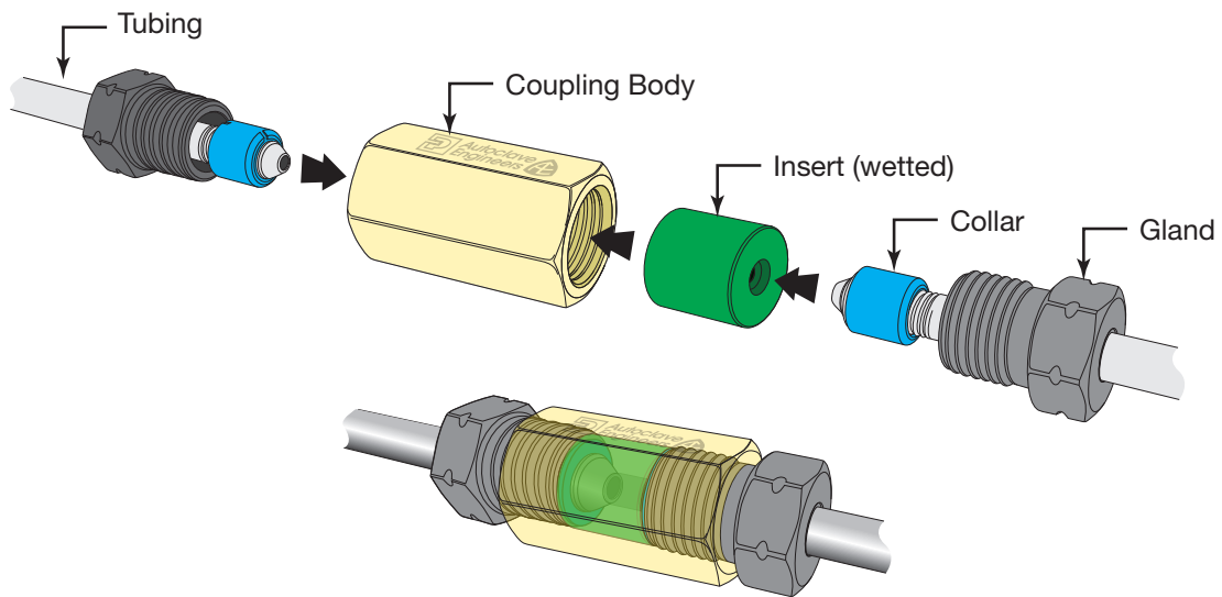
Assembled Union Coupling
