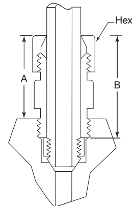
Series KCBGLX Pressures to 43,000 psi (2965 bar)
