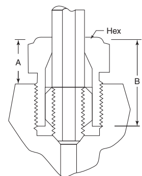
Series KCGL 60,000 psi (4140 bar)
